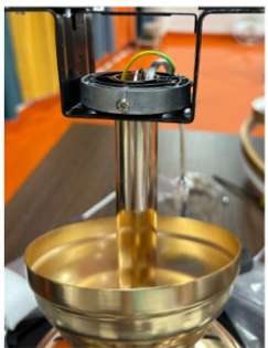
Step 13. The positioning slot on the mounting bracket of the rotary hanger has fallen into the positioning slot on the hanging ball
