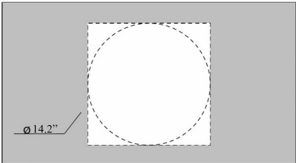
recommended cutting template \varnothing 14.2'' square 14.2" x 14.2" for tap hole
