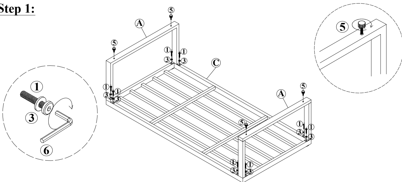
1 Bolt M6x15 - x20pcs
