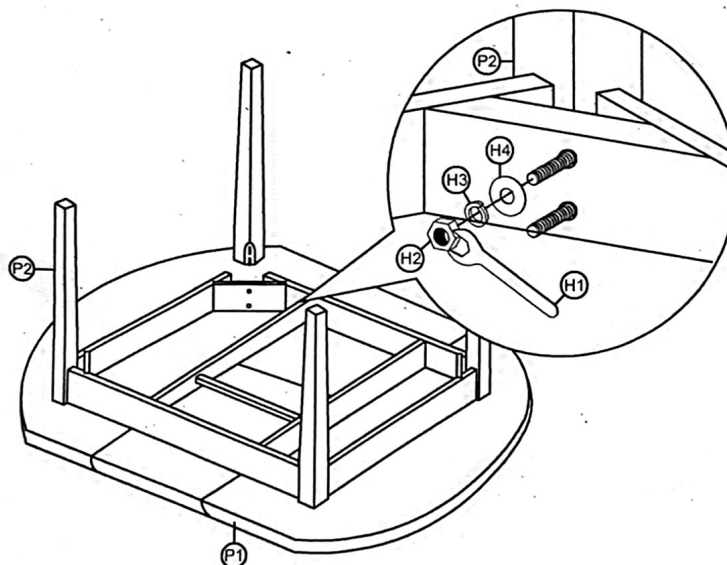
COMPLETE ASSEMBLY
