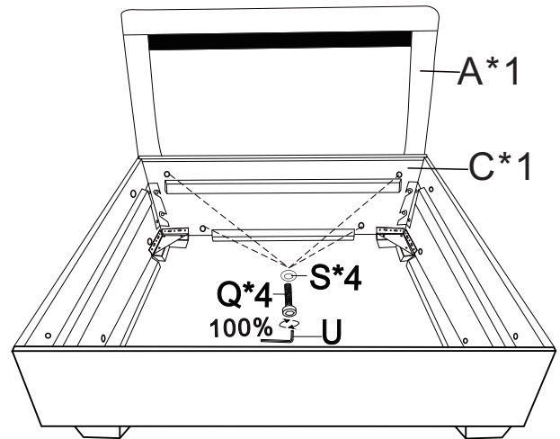
Backrest 2
