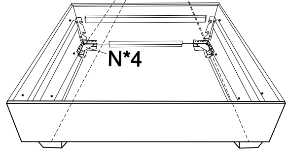
Seat frame 2
