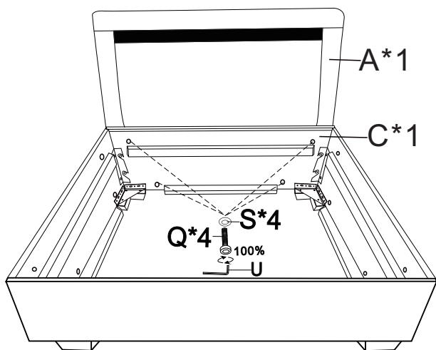
Backrest 1
