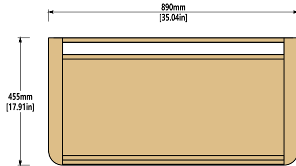
Top view of the cabinet body
