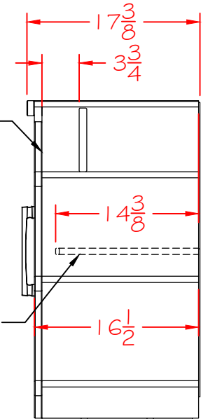
SECTIONAL VIEW
