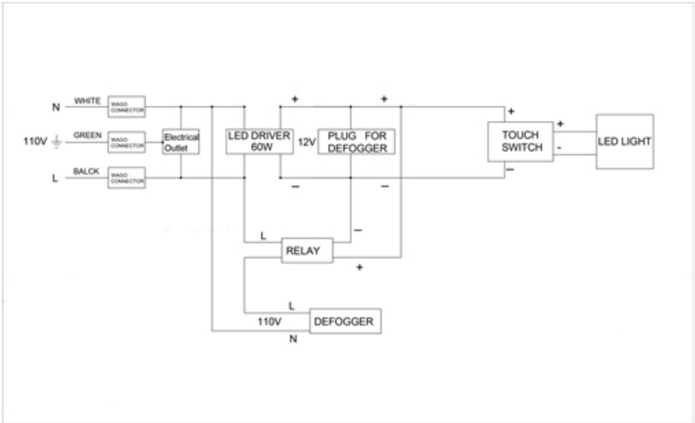
Circuit Diagram
