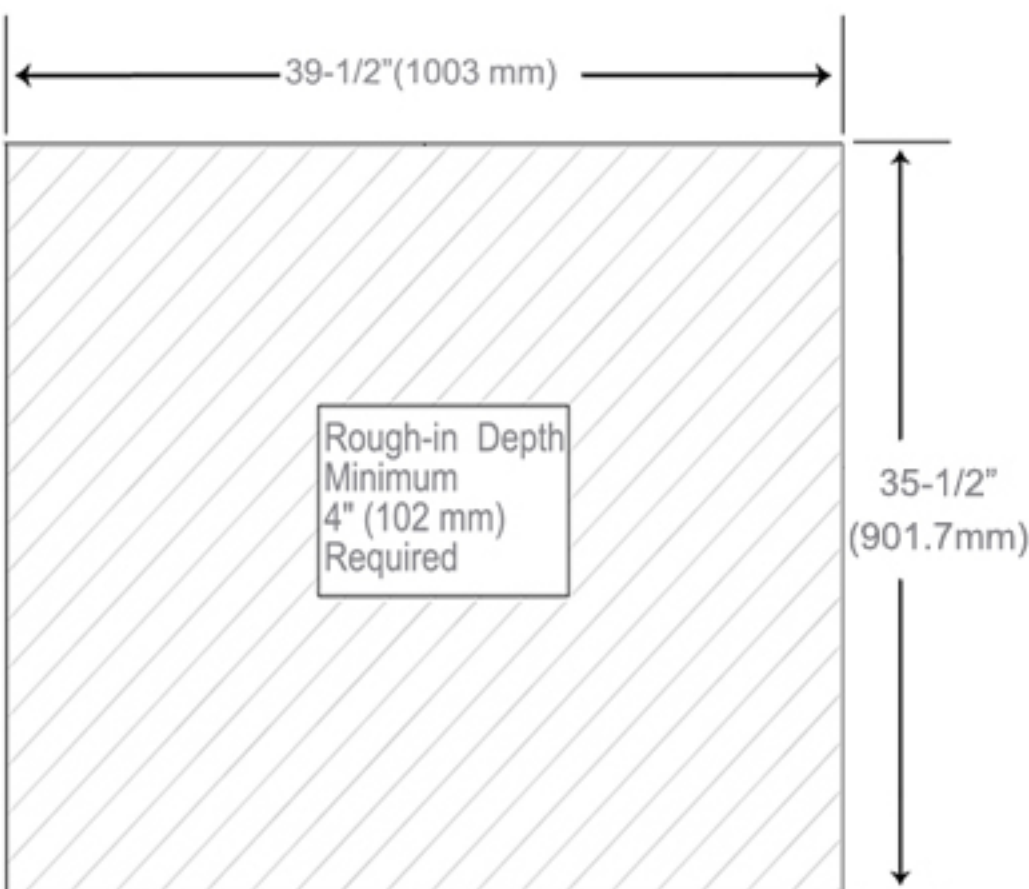
Rough-in Dimensions
