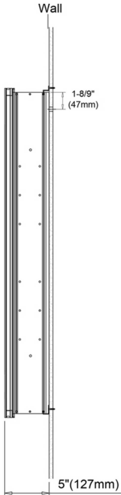
Surface Mount
