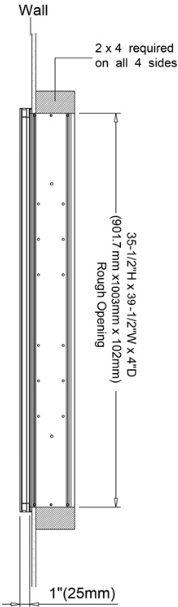
Recessed Mount
