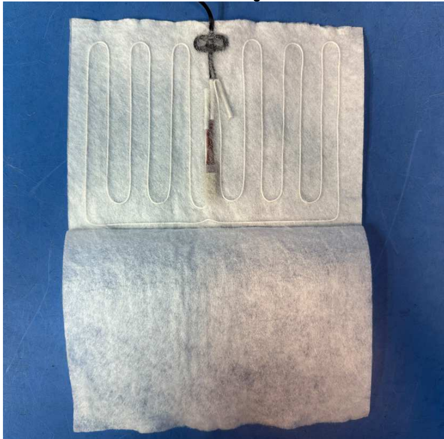
Photo 11: Internal view of Heating element for all models
