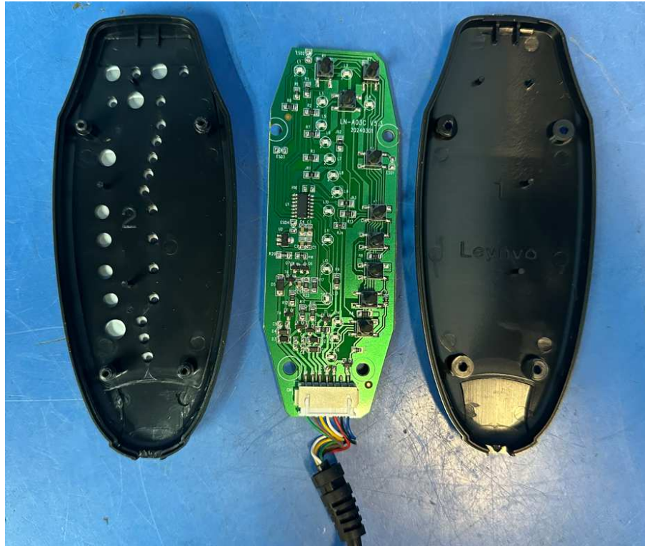
Photo 4: Internal view of controller for model LN-207-XJR
