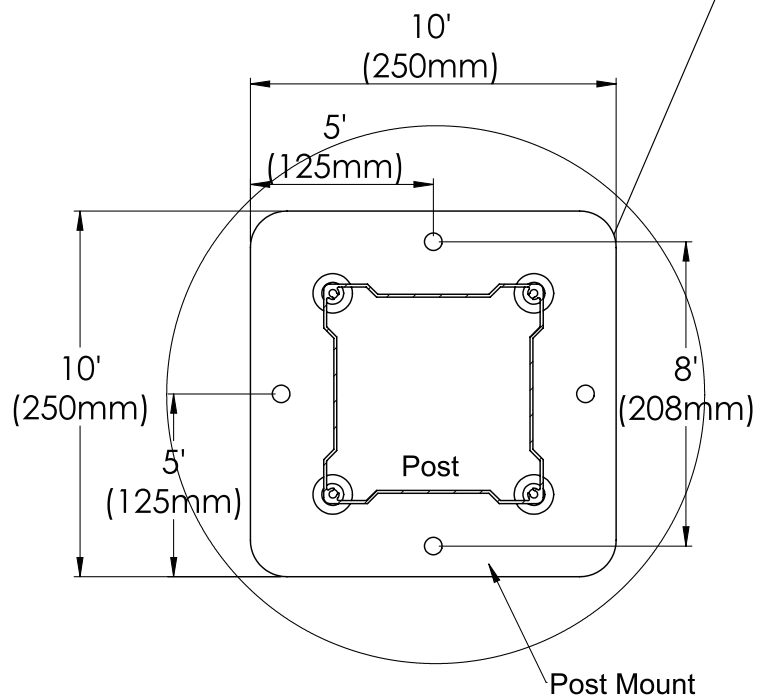
Post Detail
