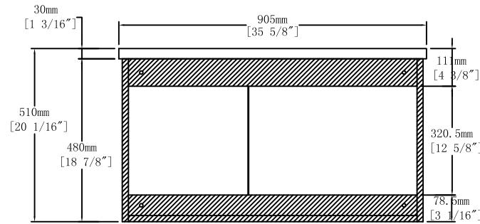
Back View
