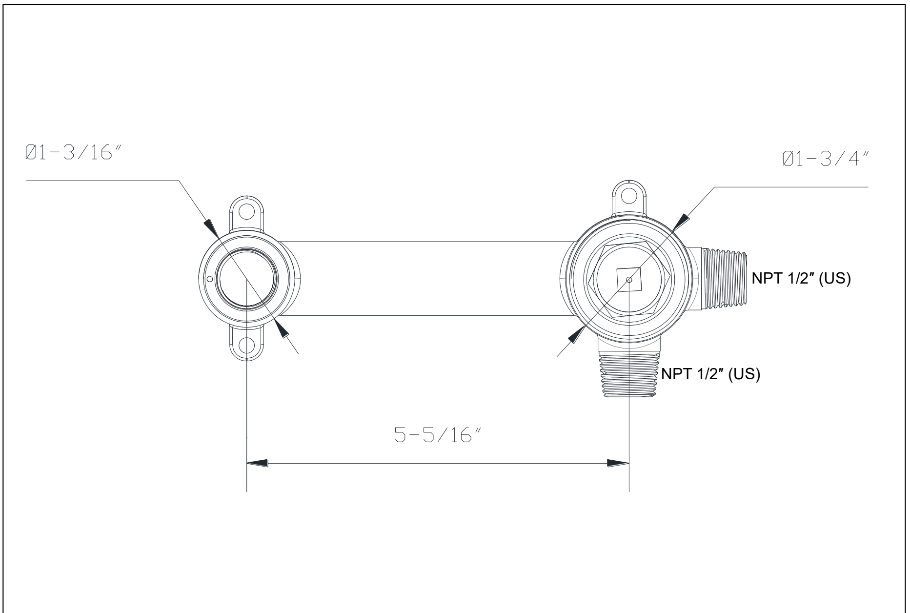
FRONT VIEW OF ROUGH IN VALVE
