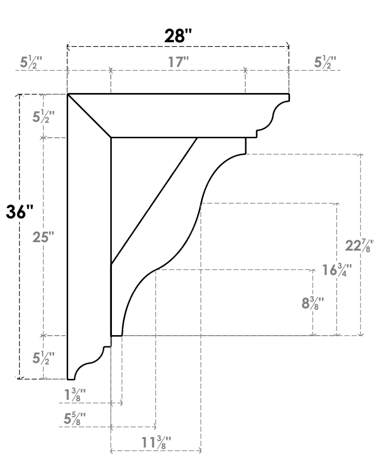
SIDE PROFILE
