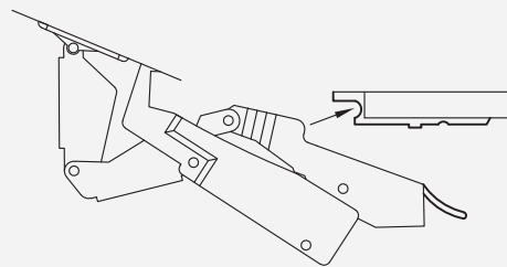
Mounting Plate
