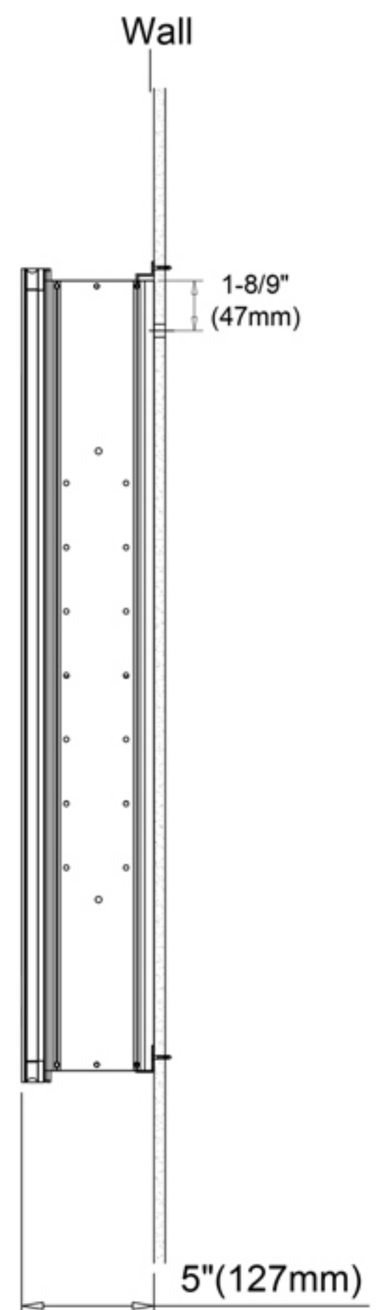
Surface Mount
