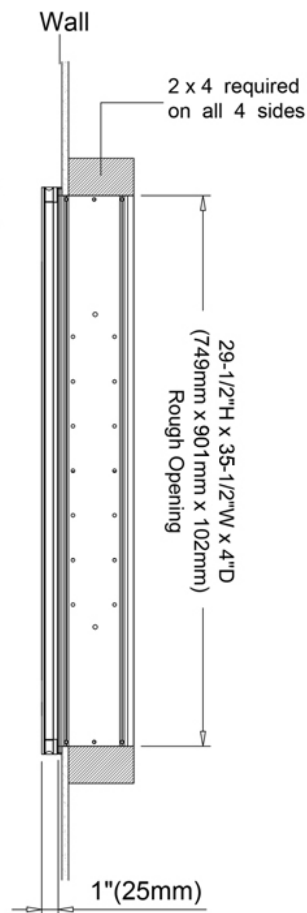
Recessed Mount
