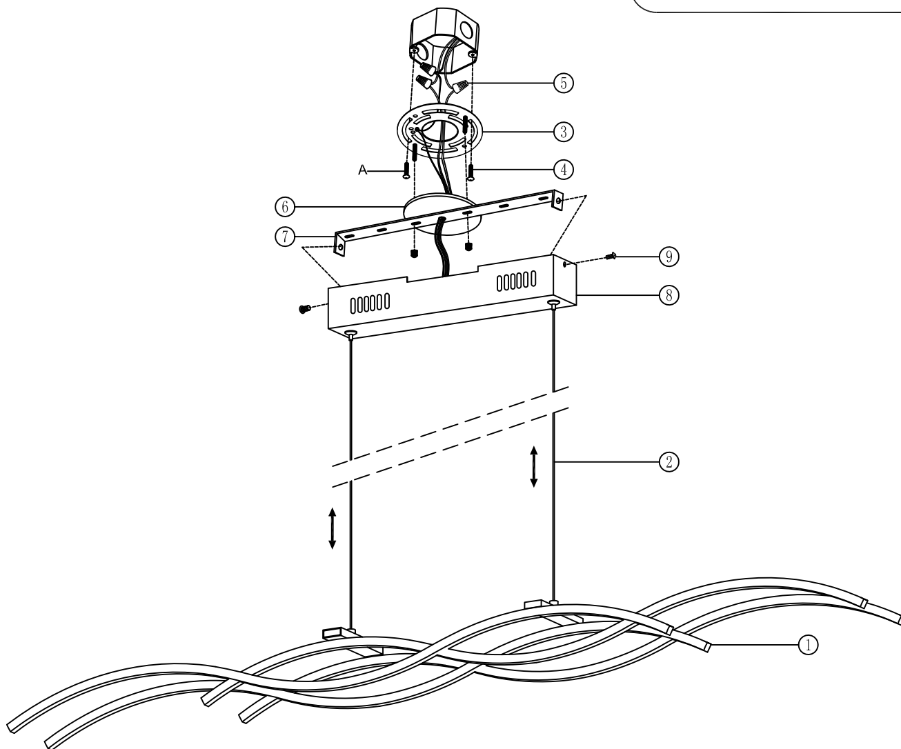
Wire connection
