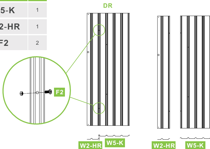
Right door panel splicing
