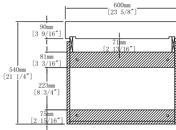
Back View
