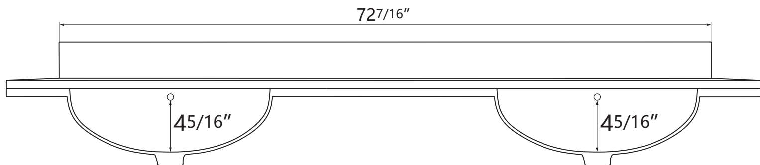
Front View
