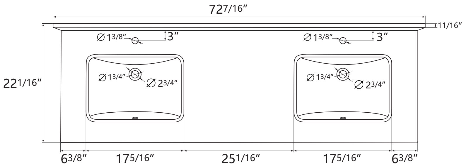
Top View
