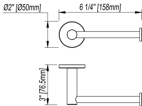
ROLL HOLDER
