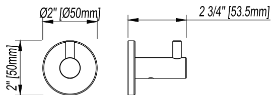
COAT HOOK
