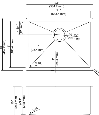
K1-S23 23"X18"X10" Min Cabinet Size: 27"
