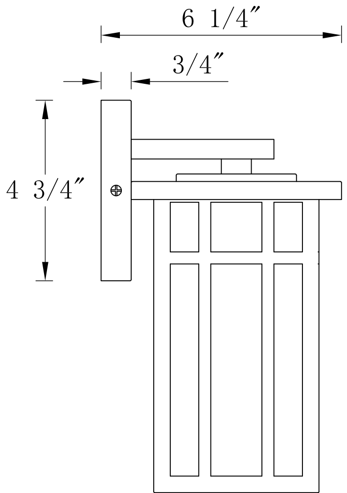
SIDE VIEW
