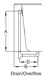
Drain/Overflow
