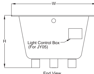
End View
