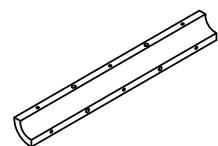
④ (490x63.6x26.2mm)X2
