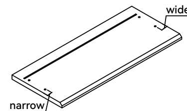
⑭ (479.5x200x15mm)X1
