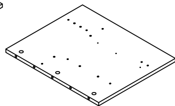
② (405x490x15mm)X1
