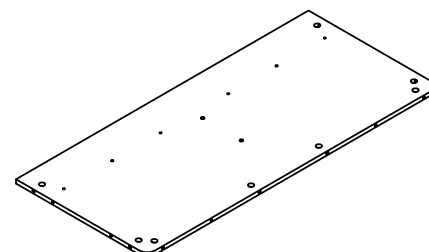
⑥ (968x434x12mm)X1
