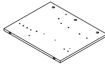
③ (405x490x15mm)X1
