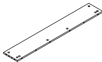
⑤ (968x156x12mm)X1
