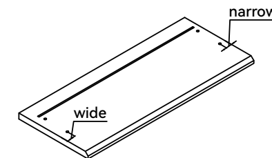
⑮ (479.5x200x15mm)X1
