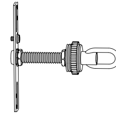
Crossbar assembly
