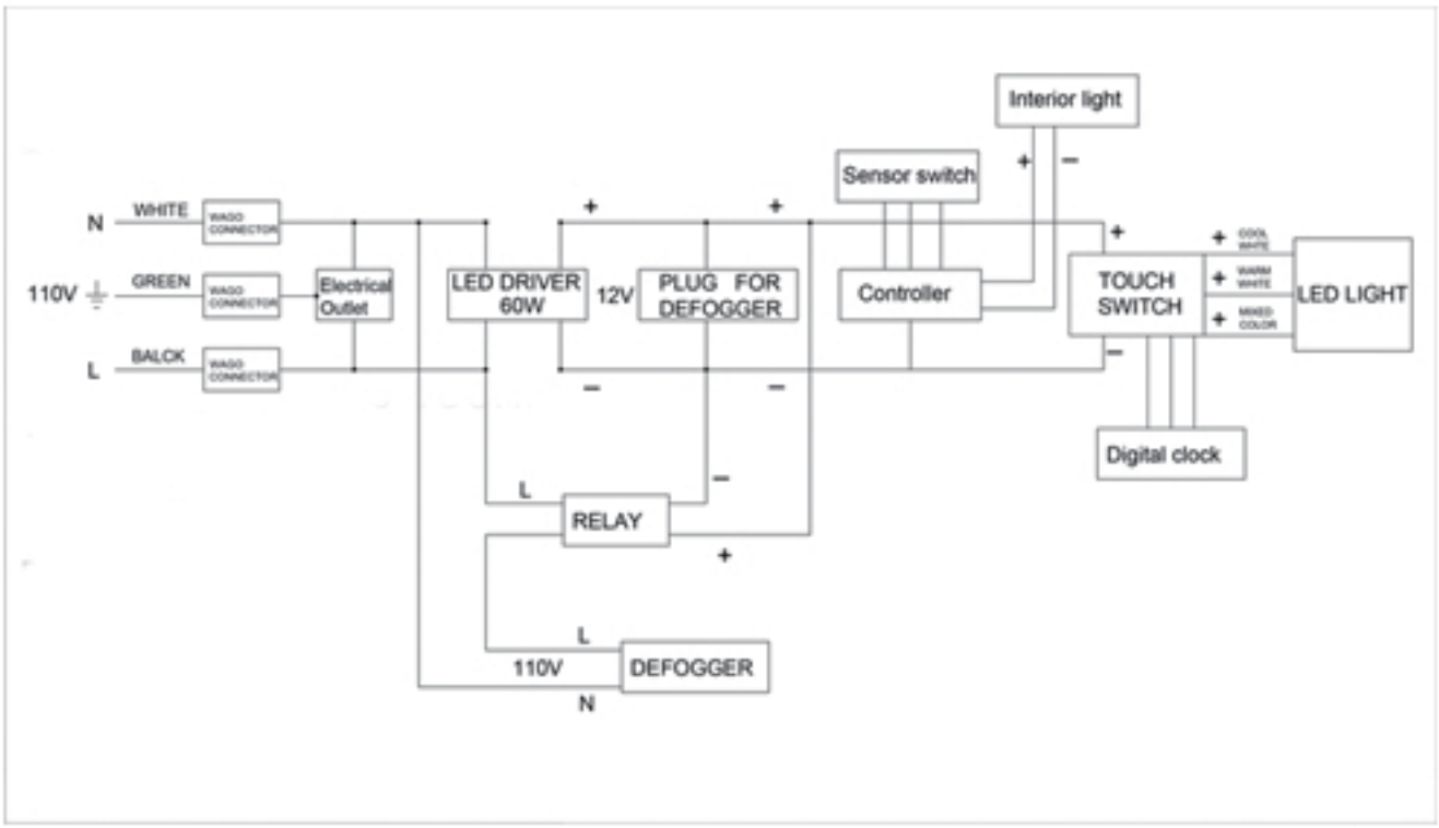
Circuit Diagram
