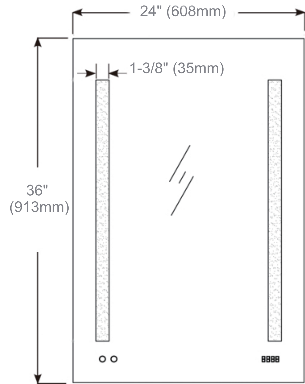
Cabinet Dimensions
