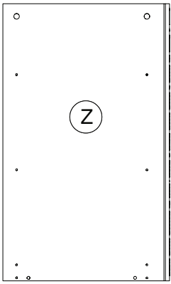
FI7423 746x450x16mm
