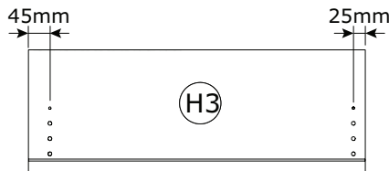
CS2768T 707x260x25mm
