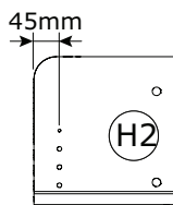
CS2544 250x260x25mm
