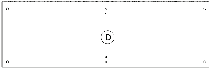
BA1938 1370x434x38mm
