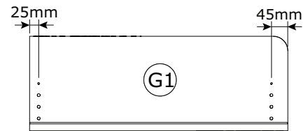
CS2770 707x260x25mm
