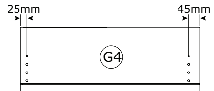
CS2760 707x260x25mm
