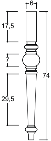
FOOT DETAIL
