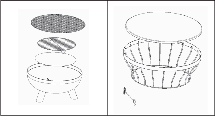
Installation diagram.
