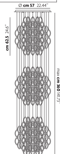
Suspension Triple Large SO3
