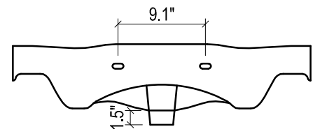
BACK VIEW
