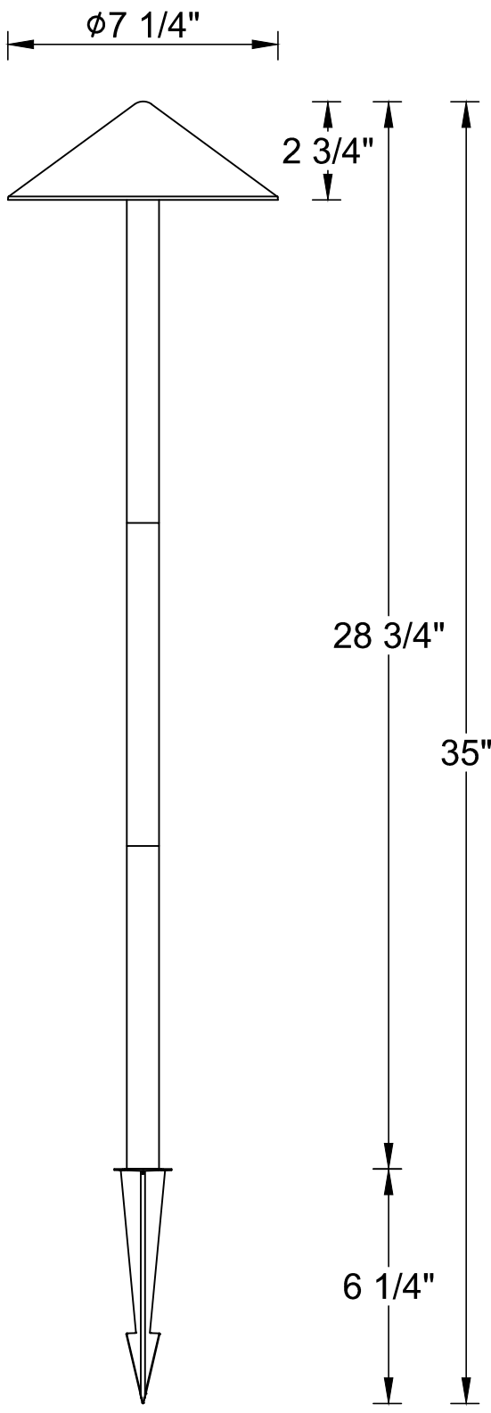
FRONT VIEW
