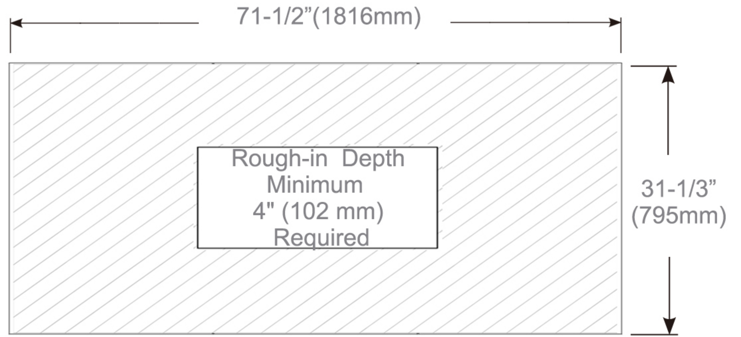
Rough-in Dimensions
