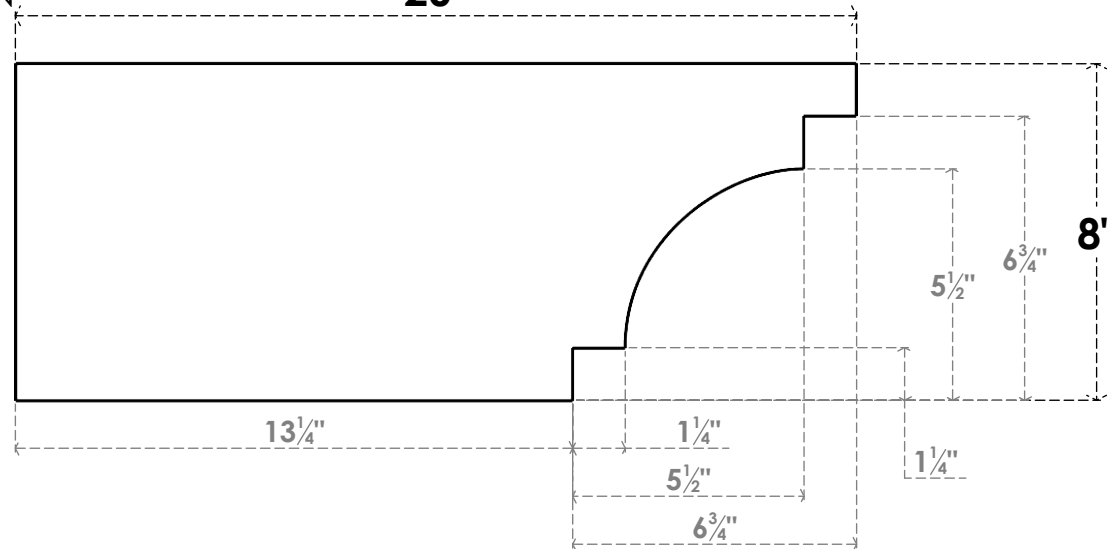
SIDE PROFILE
