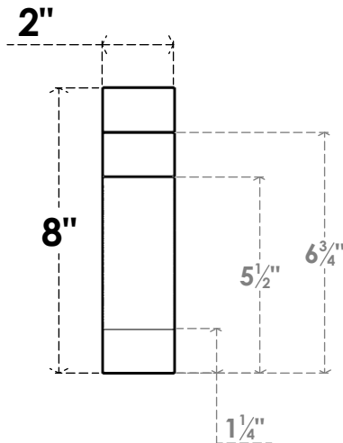
FRONT PROFILE
