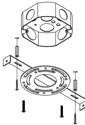
Install Metal Bracket to Ceiling
