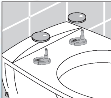
Place covering caps on the hinges
