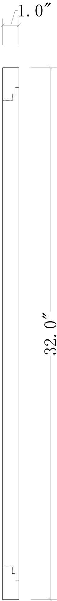
SIDE VIEW
