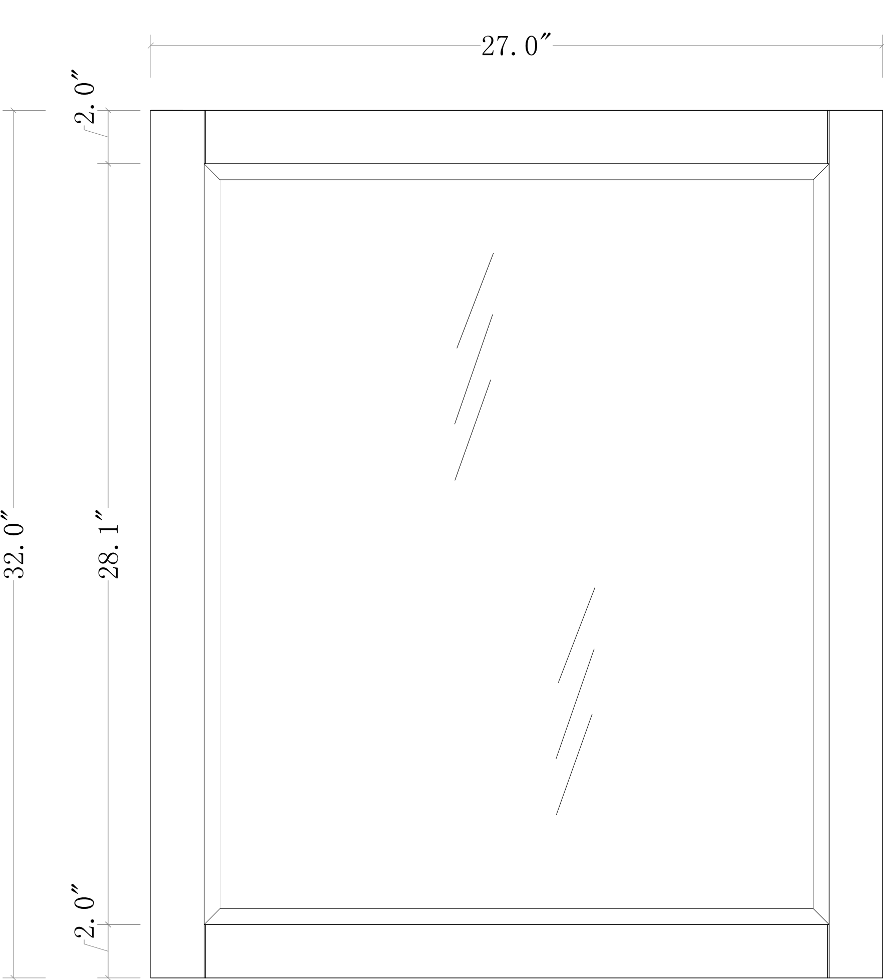
FRONT VIEW
