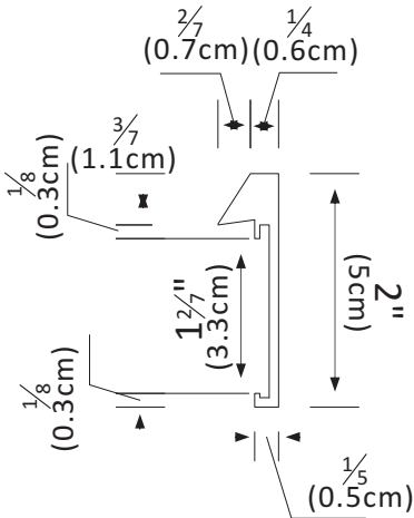
Aluminum section
