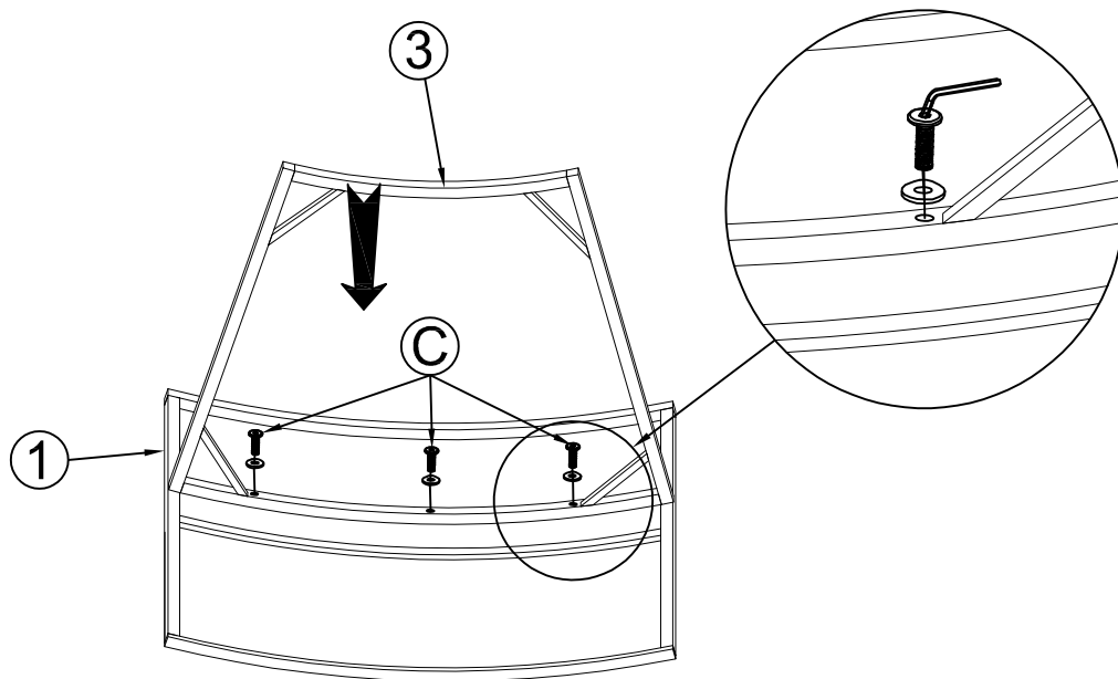
STEP 1: Connect Right Back Frame (1) and Right Seat Frame (3), tighten Allen Bolt (C), Flat Washer (E) with Allen Key (F).
