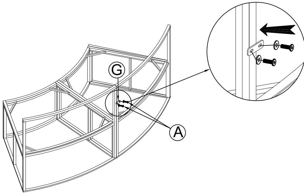
STEP 9: Connect The Part from STEP 8 & PAT (G), tighten Allen Bolt (A), Flat Washer (E) with Allen Key (F).
