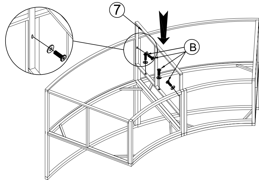
STEP 8: Connect The part from STEP 7 & Bare Frame (7), tighten Allen Bolt (B), Flat Washer (E) with Allen Key (F).
