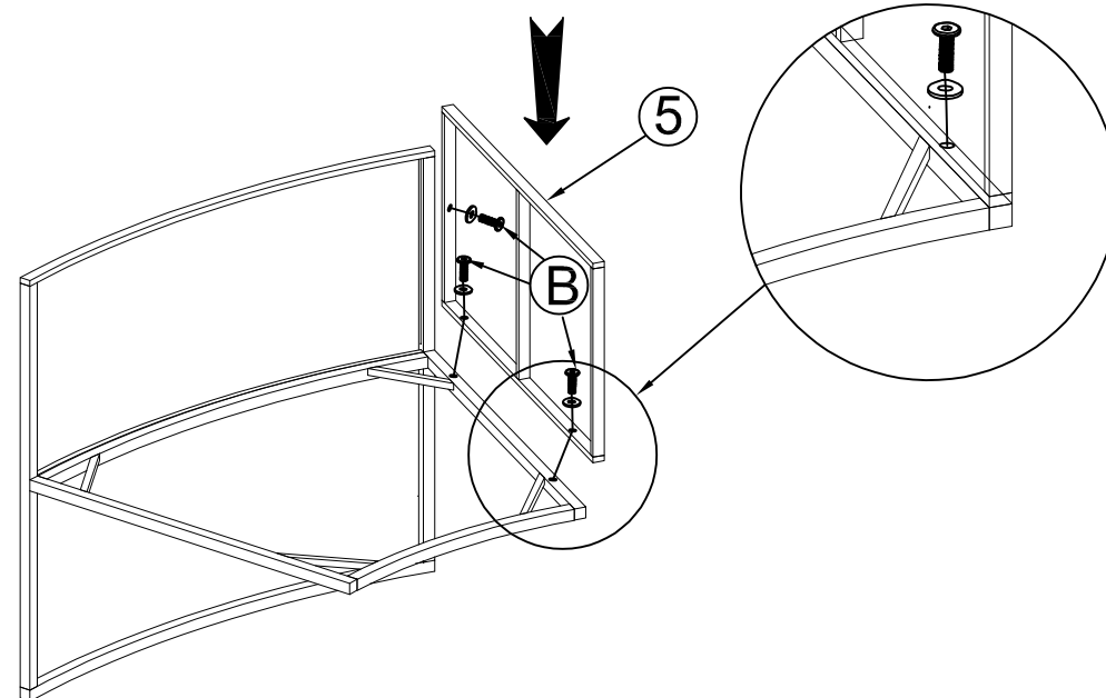
STEP 2: Connect The part from STEP 1 & Right Side Frame (5), tighten Allen Bolt (B), Flat Washer (E) with Allen Key (F).
