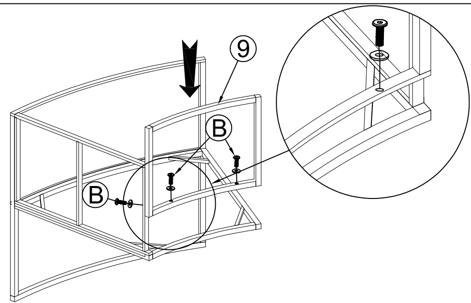
STEP 6: Connect The part from STEP (5) & Left Panel Frame (9), tighten Allen Bolt (B), Flat Washer (E) with Allen Key (H) to finish Left Chair.
