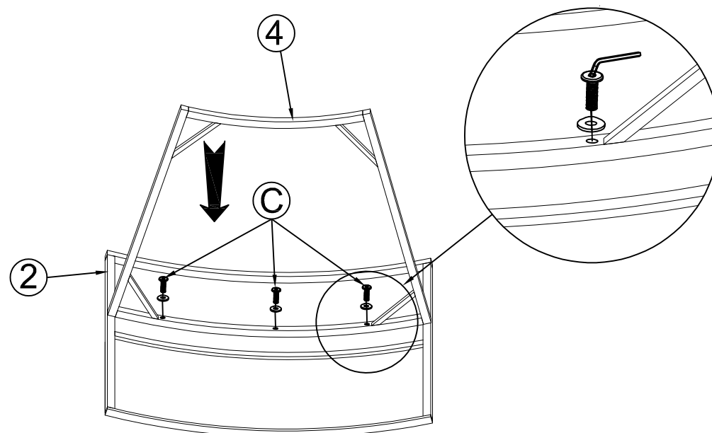
STEP 4: Connect Left Back Frame (2) & Left Seat Frame (4), tighten Allen Bolt (C), Flat Washer (E) with Allen Key (H).
