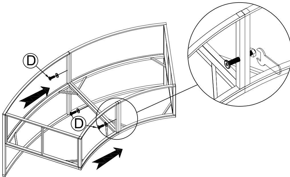
STEP 7: Connect The part from STEP 3 (Right Chair) & The part from STEP 6 (Left Chair), tighten Allen Bolt (D), Ecrú with Key (D).
