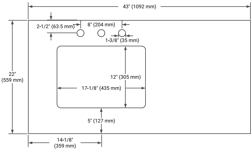
COUNTERTOP PLAN VIEW
