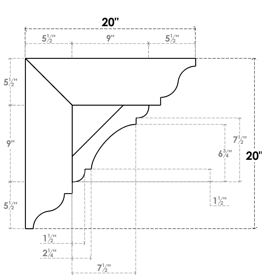
SIDE PROFILE
