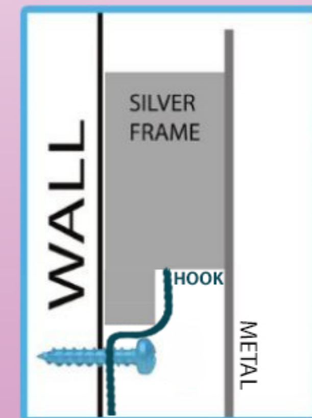
Lip for hanging over screws
