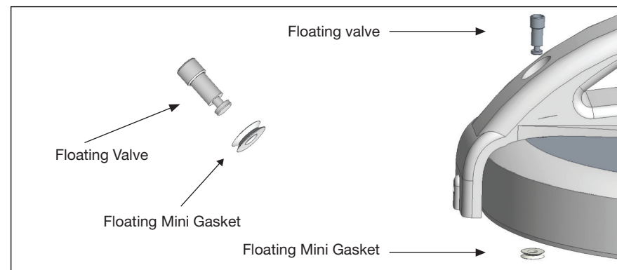
Figure: Floating valve Installation Insert the floating valve from the top of the lid and secure it in place with the washer from the bottom of the lid.
