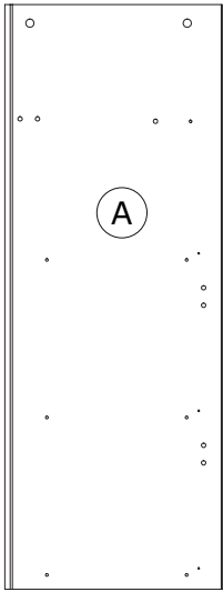
FI8827 1069x398x25mm
