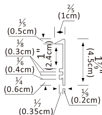
Aluminum section
