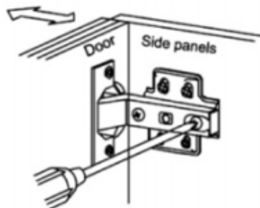
In-and-Out by loosening the hinge-arm mounting screw or via cam adjustment
