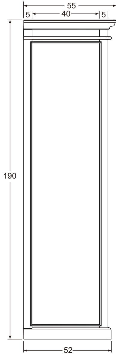
SIDE VIEW
