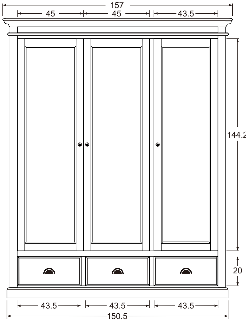
FRONT VIEW
