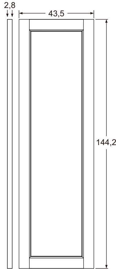
MEDIUM DOOR DETAIL
