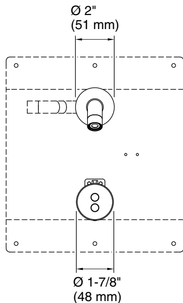
Valve Mounting Plate (not included)
