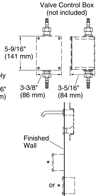
*Valve Control Box Mounting Options
