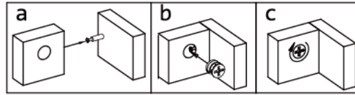
Cam Lock Fastening System
