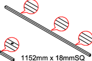
Cross Tube
