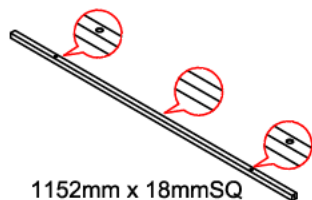
Cross Tube
